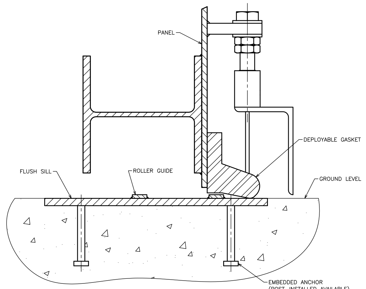
TYPICAL BOTTOM SECTION
