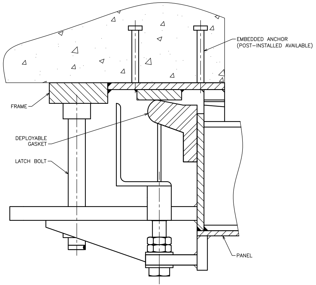
TYPICAL JAMB SECTION
