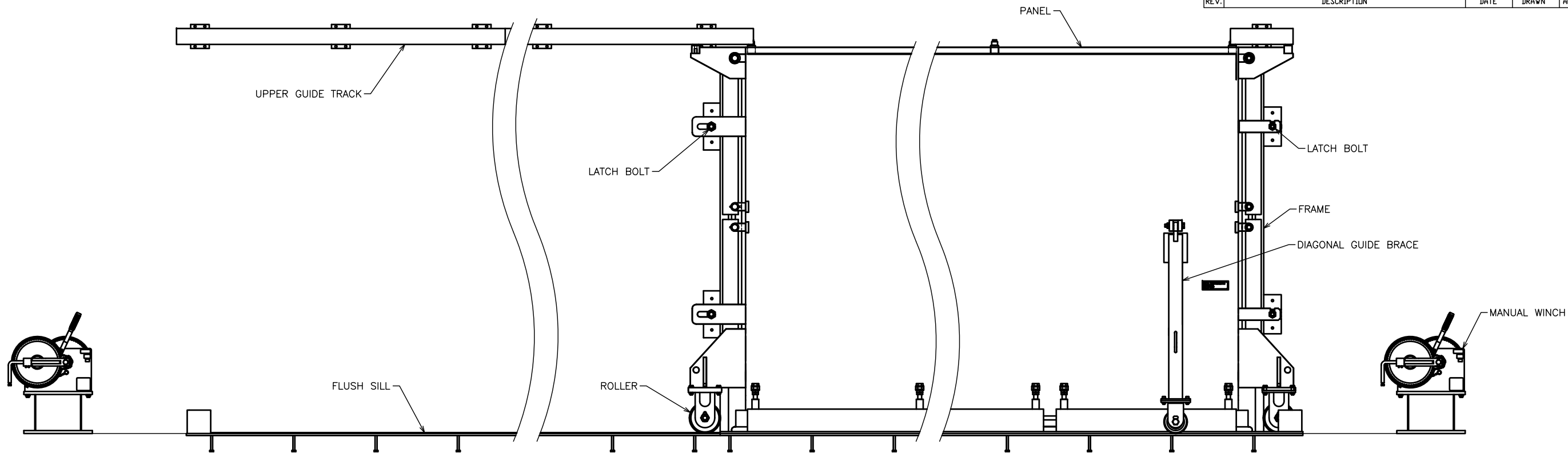
ELEVATION VIEW
